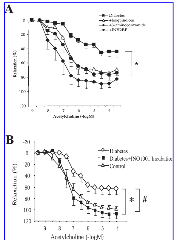
FIG. 4. In vitro treatment with all PARP inhibitors improved the endothelium-dependent relaxant ability of the diabetic vessels. (A) Endothelium-dependent relaxations induced by acetylcholine in control (nondiabetic) male Balb/c mice and 4 weeks after STZ-induced diabetes. In a subgroup of the vascular rings, evaluation of vascular responsiveness was preceded by 1-h incubation with three structurally different PARP inhibitors: 3-aminobenzamide (3 mmol/L), 5-iodo-6-amino-1,2-benzopyrone (INH2BP) (100 \mu mol/L), or 1,5-dihydroxyisoquinoline (Isoquinolone) (30 \mu mol/L). There was a marked and selective impairment of the endothelium-dependent relaxant ability of the vascular rings in diabetes at 4 weeks. In vitro treatment with all PARP inhibitors improved the endothelium-dependent relaxant ability of the diabetic vessels. * p < 0.05 for differences between experimental groups, as indicated. n = 8 per group. Reproduced with permission from 91. (B) Endothelium-dependent relaxations induced by acetylcholine in control (nondiabetic) male Balb/c mice and 6 weeks after STZ-induced diabetes. In a subgroup of the vascular rings, evaluation of vascular responsiveness was preceded by 1-h incubation with the novel potent PARP inhibitor, INO1001 (3 \mu mol/L). There was a marked and selective impairment of the endothelium-dependent relaxant ability of the vascular rings in diabetes at 6 weeks. In vitro treatment with all PARP inhibitors improved the endothelium-dependent relaxant ability of the diabetic vessels. #, * p < 0.05 for differences between experimental groups, as indicated. n = 8 per group.
