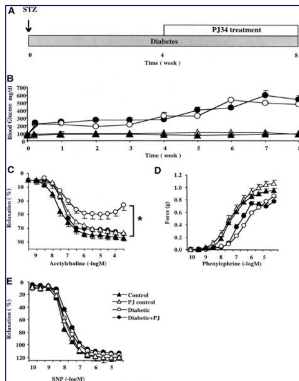
FIG. 3. Pharmacological inhibition of PARP restores impaired endothelium-dependent relaxant ability of the diabetic vessels. Blood glucose levels and vascular responsiveness are presented. Endothelium-dependent relaxations were induced by acetylcholine, contractions induced by phenylephrine, and endothelium-independent relaxations induced by sodium nitroprusside (SNP) in control (nondiabetic) male Balb/c mice and 1, 4, and 8 weeks after STZ-induced diabetes. Vehicle or PARP inhibitor (PJ34, 10 mg/kg oral gavage once a day) treatment started at 4 weeks after STZ and continued until 8 weeks (the end of the experimental period). There was a marked and selective impairment of the endothelium-dependent relaxant ability of the vascular rings in diabetes at 4 and 8 weeks. Treatment with the PARP inhibitor between weeks 4 and 8 restored to normal the endothelium-dependent relaxant ability of the diabetic vessels despite the persistence of hyperglycemia. * p < 0.05 for differences between experimental groups, as indicated. n = 8 per group. Reproduced with permission from 91.
