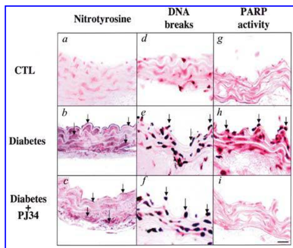
FIG. 1. Reactive nitrogen species generation, DNA breakage, and PARP activation in diabetic blood vessels. (a–c) Immunohistochemical staining for nitrotyrosine in control rings (a), in rings from diabetic mice treated with vehicle at 8 weeks (b), and in rings from diabetic mice treated with PJ34 (c). (d–f) Terminal deoxyribonucleotidyl transferase-mediated dUTP nick-end labeling, an indicator of DNA-strand breakage, in control rings (d), in rings from diabetic mice treated with vehicle at 8 weeks (e), and in rings from diabetic mice treated with PJ34 (f). (g–i) Immunohistochemical staining for poly(ADP-ribose), an indicator of PARP activation, in control rings (g), in rings from diabetic mice treated with vehicle at 8 weeks (h), and in rings from diabetic mice treated with PJ34 (i). Reproduced with permission from 33.
