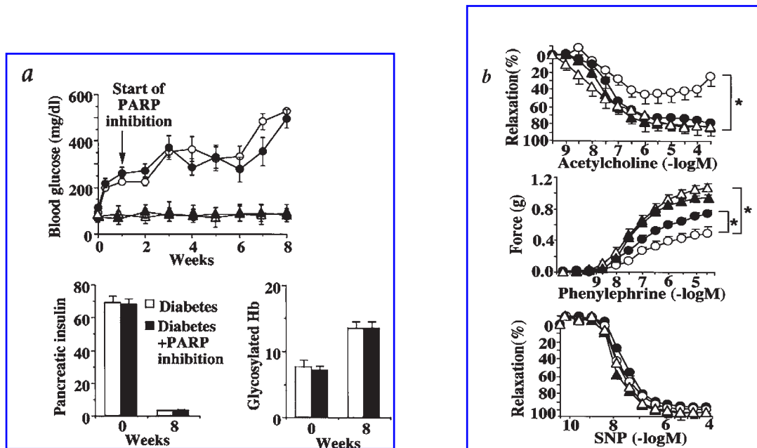
FIG. 2. Reversal of diabetes-induced endothelial dysfunction by pharmacological inhibition of PARP. The following symbols were used for the respective groups: animals that received no STZ injection ( \Delta ), nondiabetic control animals at 8 weeks treated with PJ34 between week 1 and 8 ( \blacktriangle ), diabetic animals at 8 weeks treated with vehicle ( \circ ), diabetic animals at 8 weeks treated with PJ34 between week 1 and 8 ( \bullet ). (a) Blood glucose levels, pancreatic insulin content (ng of insulin/mg of pancreatic protein), and blood glycosylated hemoglobin (Hb) (expressed as % of total Hb) at 0–8 weeks in nondiabetic, control male BALB/c mice, and at 0–8 weeks after STZ treatment (diabetic) in male BALB/c mice. PARP inhibitor treatment, starting at 1 week after STZ and continuing until the end of week 8, is indicated by the arrow. Pancreatic insulin and glycosylated hemoglobin levels are shown at 8 weeks in vehicle-treated and STZ-treated animals, in the presence or absence of PJ34 treatment. (b) Acetylcholine-induced, endothelium-dependent relaxations, phenylephrine-induced contractions, and sodium nitroprusside (SNP)-induced endothelium-independent relaxations. * p < 0.05 for vehicle-treated diabetic versus PJ34-treated diabetic mice ( n = 8 per group). Reproduced with permission from 33.
