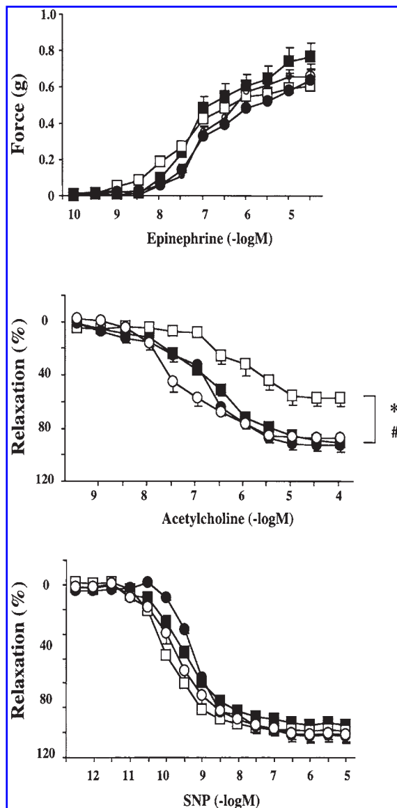
FIG. 5. Reversal of diabetes-induced endothelial dysfunction by pharmacological inhibition of PARP in diabetic NOD mouse vascular rings. Epinephrine-induced contractions ( upper panel ), acetylcholine-induced endothelium-dependent relaxation ( middle panel ), and sodium nitroprusside (SNP)-induced endothelium-independent relaxations ( lower panel ). ■, control; ○, control + PJ34; □, diabetes; ●, diabetes + PJ34. Each point of the curve represents the mean \pm SE of five to eight experiments in vascular rings. * p < 0.05 versus control; # p < 0.05 versus diabetes. Reproduced with permission from 72.
